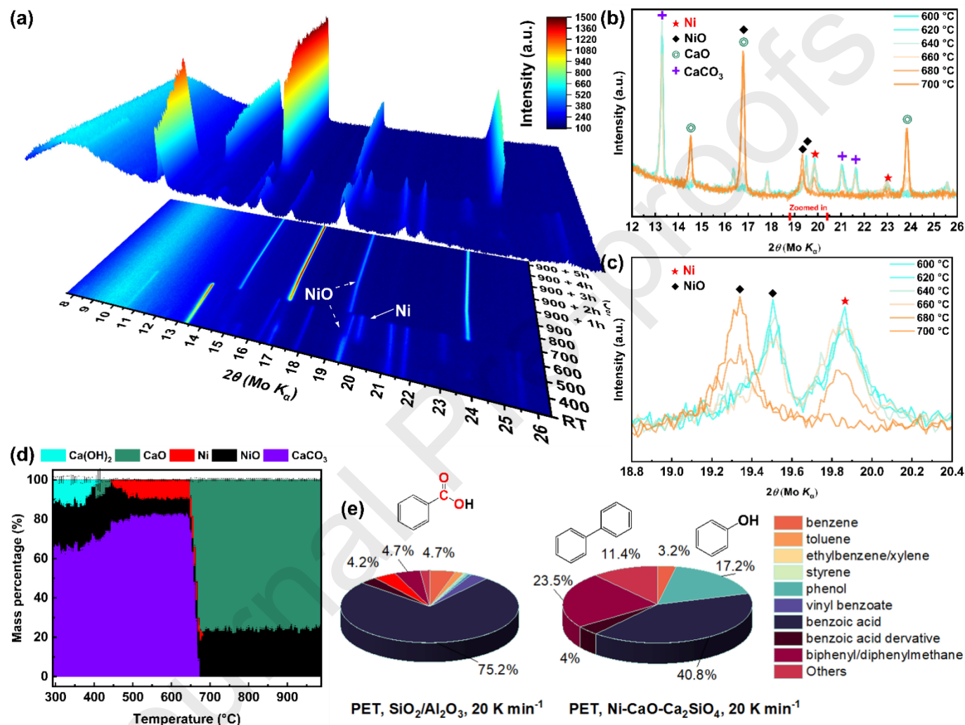
Fig 6. (a, b) In situ PXRD patterns of Ni-CaO-Ca 2 SiO 4 , PET loaded, N 2 flow, 20 °C min -1 ramping rate, with scans every 5 °C, hold at 900 °C for 6 h with scans every 2.5 min. (c) zoomed-in view of (b) to demonstrate the reduction of NiO. (d) Calculated mass evolution of catalyst in (a). (e) Distribution of pyrolysis products collected from for the experiments conducted by a Py-GCMS with PET mixed with SiO 2 /Al 2 O 3 and Ni-CaO-Ca 2 SiO 4 , respectively.
