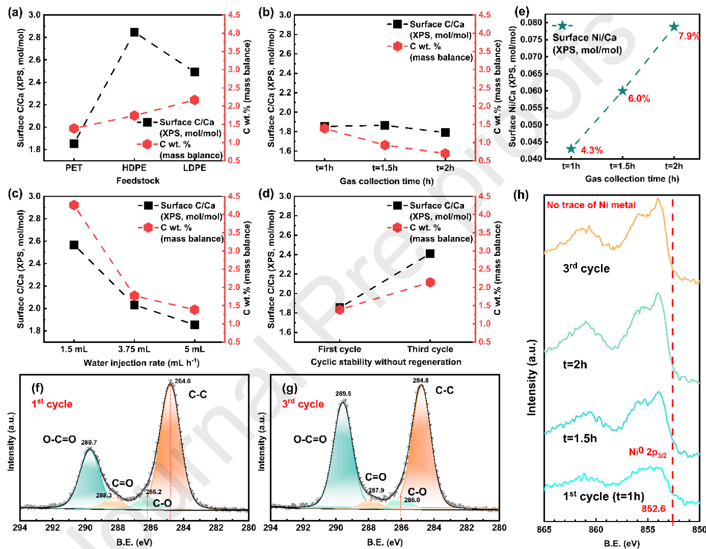
Fig. 4. Surface C/Ca molar ratio by XPS and carbon wt.% by mass balance for spent catalysts with relative parameters (a–d). (e) Surface Ni/Ca molar ratio by XPS for (b). (f, g) C 1s XPS spectra for spent catalysts after the 1st and 3rd cycles. (h) Ni 2p XPS spectra for spent catalysts.
