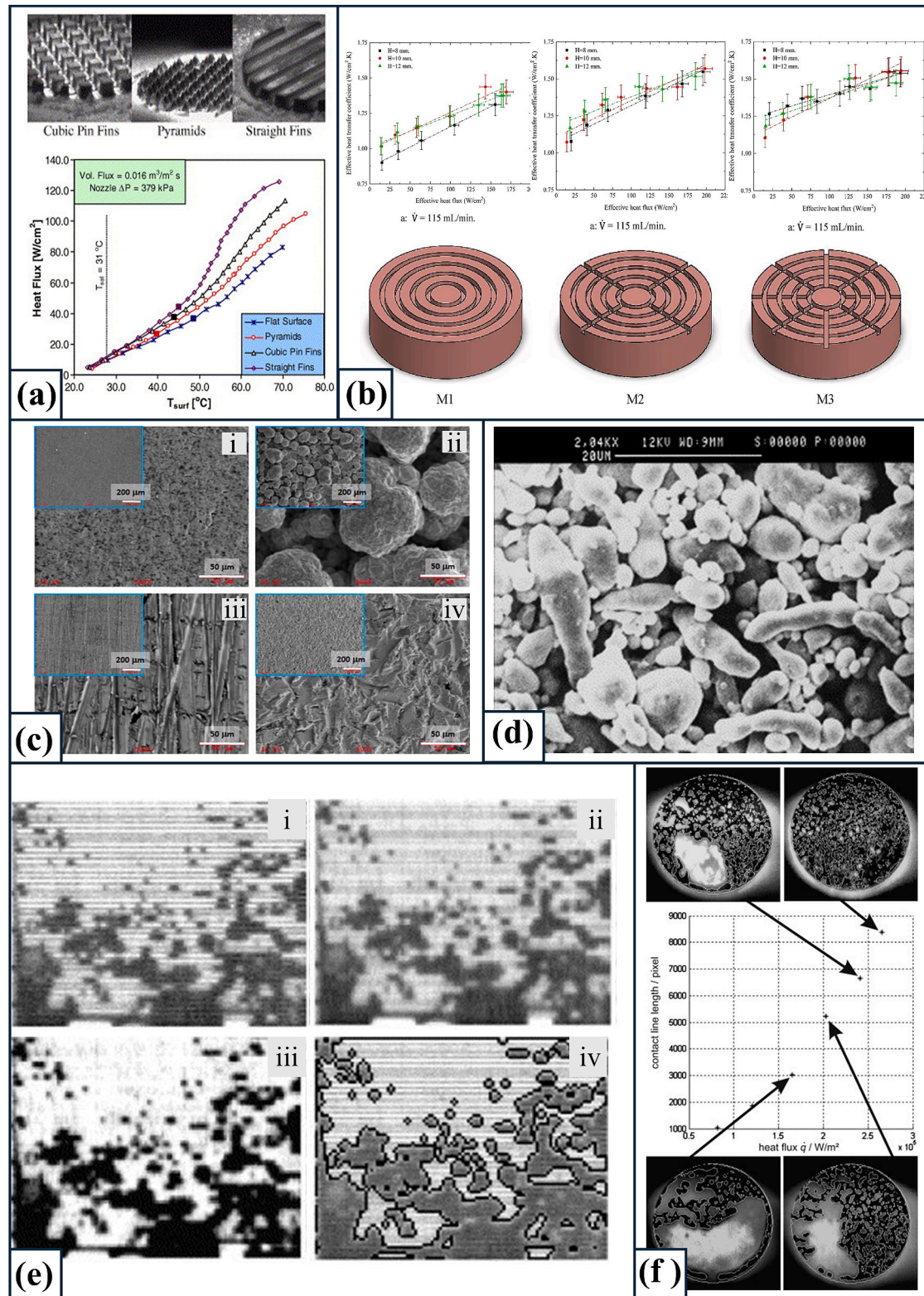
Fig. 14. Effects of surface microstructures on conventional spray cooling. (a) Images of square pin fin, pyramid, and straight fin enhanced surfaces, and plots of heat flux versus surface temperature. Reprinted from Ref. [129] with permission from Elsevier (License No. 6194331448190); (b) CAD images of M1, M2, and M3 structured surfaces, and the effect of nozzle-to-surface distance on effective heat flux for M1, M2, and M3 surfaces at a flow rate of 115 mL/min. Reprinted from Ref. [131] with permission from Elsevier (License No. 6194340307346); (c) SEM images of surfaces: (i) RS, (ii) SS, and (iv) BS at 100x and 500x magnifications. Reprinted from Ref. [132] with permission from Elsevier (License No. 6194340541760); (d) SEM image of the ABM coating. Reprinted from Ref. [133] with permission from Elsevier (License No. 6194340729030); (e) Image processing sequence: (i) raw image, (ii) application of a 2-pixel orthogonal filter, (iii) row-by-row renormalization, and (iv) final detected edges superimposed on the raw image. Reprinted from Ref. [134] with permission from Elsevier (License No. 6194341039305); (f) Contact line length versus heat flux and corresponding infrared images. Reprinted from Ref. [135] with permission from Elsevier (License No. 6194341240862).
