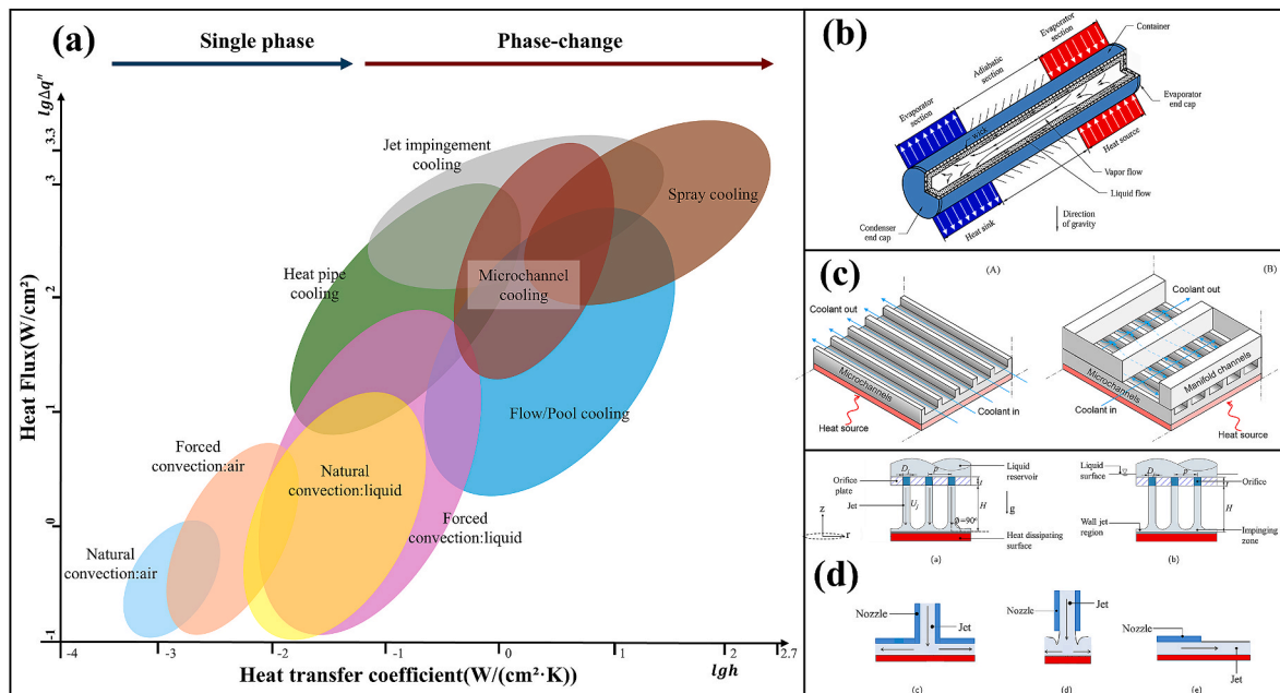
Fig. 1. Overview and mechanism of various advanced cooling technologies. (a) Comparative analysis of heat transfer performance under different cooling technologies. Reprinted from Ref. [36], Copyright [2022], by ASME; (b) Heat pipe cooling device [37]; (c) Microchannel cooling. Reprinted from Ref. [38] with permission from Elsevier (License No. 6194250072879); (d) Jet impingement cooling. Reprinted from Ref. [39] with permission from Elsevier (License No. 6194240710129).
